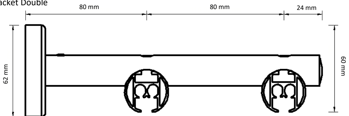
CRS Wall Bracket Double
